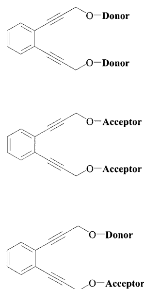
Figure 1. Representation of donor–acceptor-containing enediynyl compounds.
