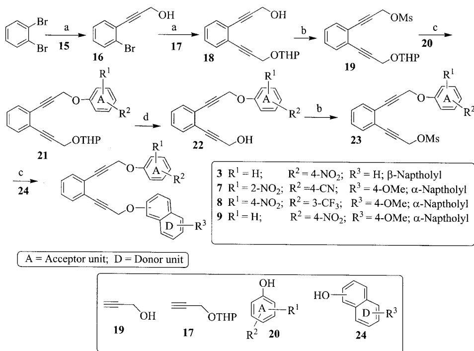
Scheme 1. Synthesis of naphthoxy-based D/A enediynes. Reagents and conditions: a) Pd 0 , n BuNH 2 , propargyl alcohol/THP-protected propargyl alcohol; b) MesCl/CH 2 Cl 2 ; c) K 2 CO 3 /DMF; d) PPTS/EtOH.
