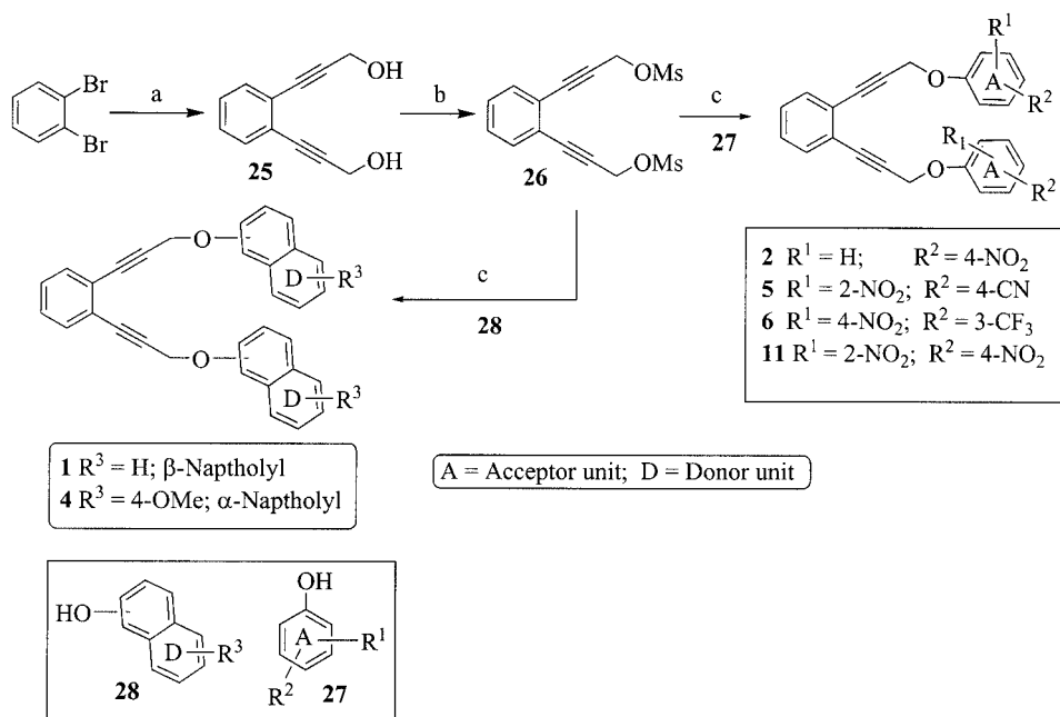
Scheme 2. Synthesis of D/D and A/A enediynes. Reagents and conditions: a) Pd 0 , n BuNH 2 , propargyl alcohol; b) MesCl/CH 2 Cl 2 ; c) K 2 CO 3 /DMF/27 or 28.
